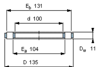
Roller and cage thrust assembly
