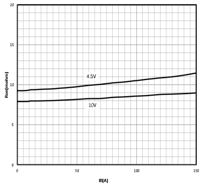
Typ. drain-source on resistance
