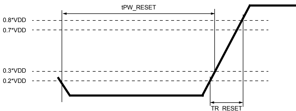
RESET_n Input Slew Rate Definition
