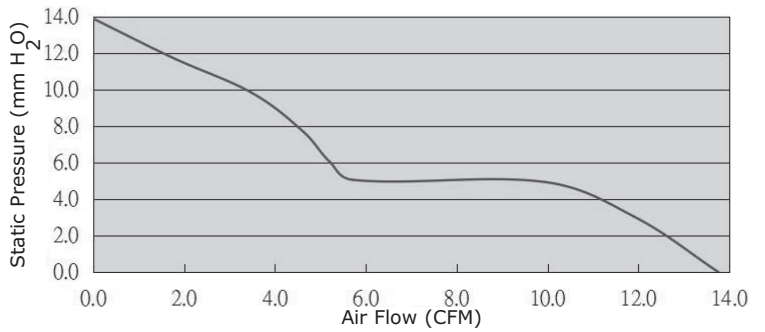
CFM-4020BF-2110-381
