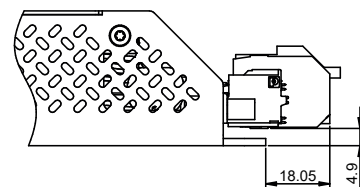
Fig. 10 Plugged connector for RCM200/300 with option K
