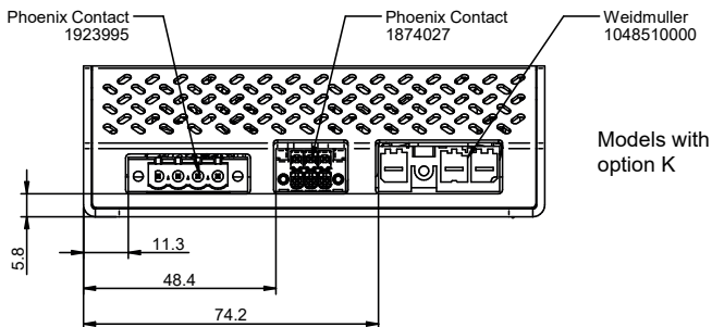
Fig. 9 Case of RCM200/300 (RCM02) weight approx. 820 g, Aluminum, EP-powder coated
