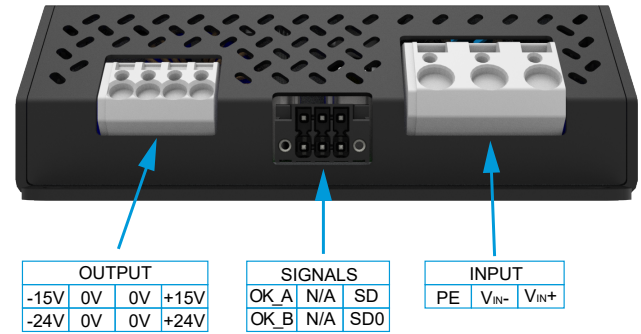
Fig. 11 Pin allocation of RCM200/300
