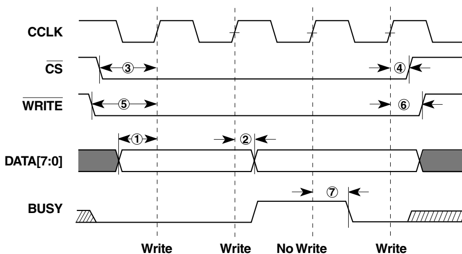
Figure 16: Write Operations
