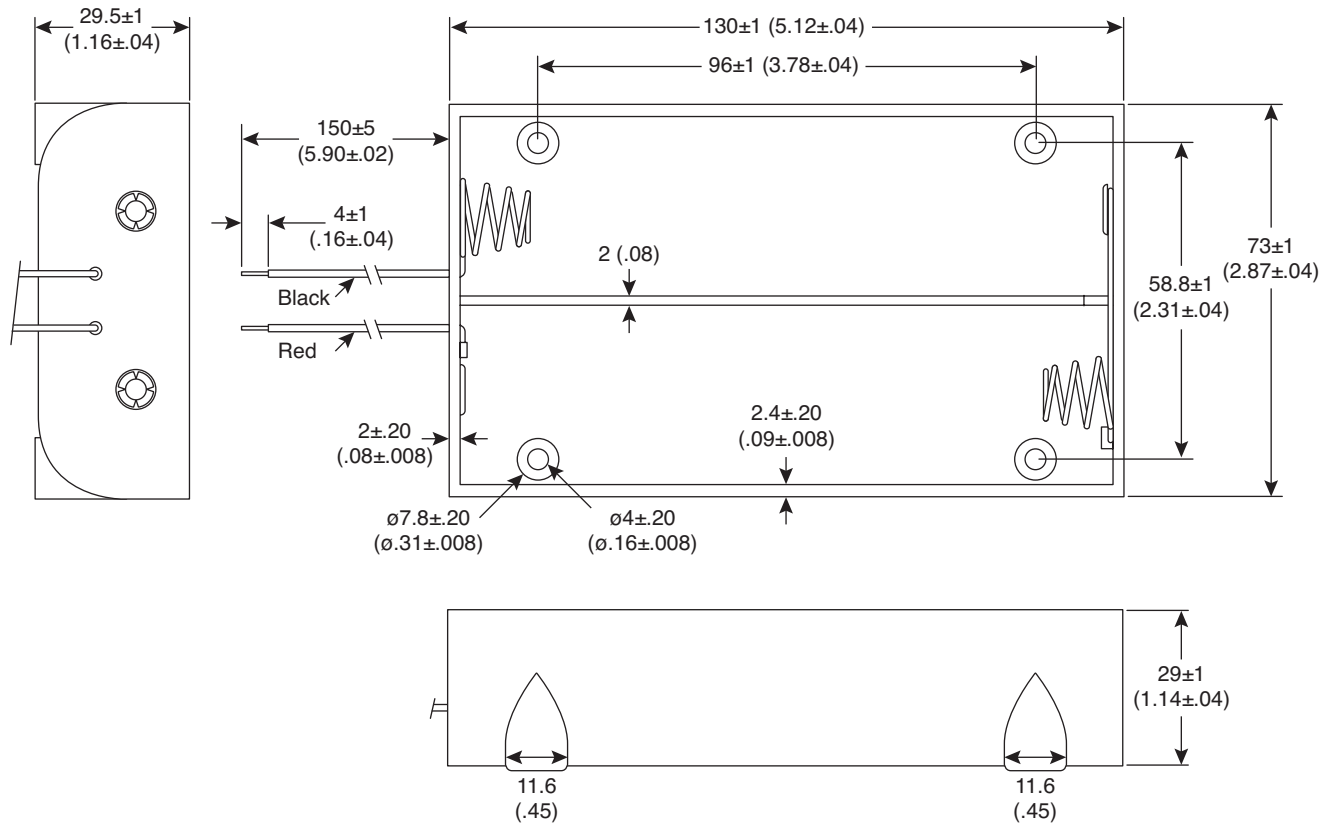
DIMENSIONS: mm (in.)
