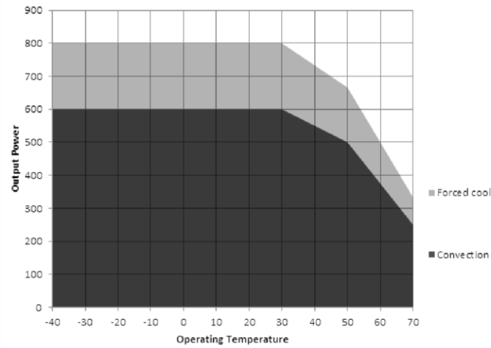
Figure 3. Power Derating Curve 24 V and above
