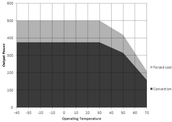
Figure 2. Power Derating Curve 15 V
