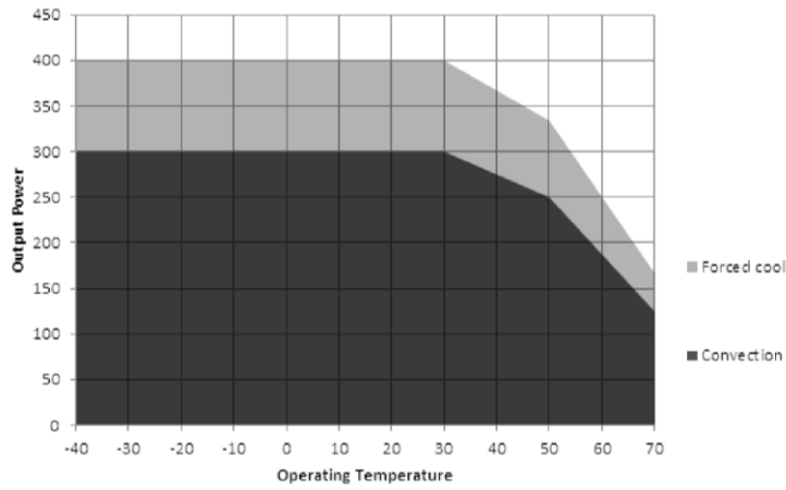
Figure 1. Power Derating Curve 12 V
