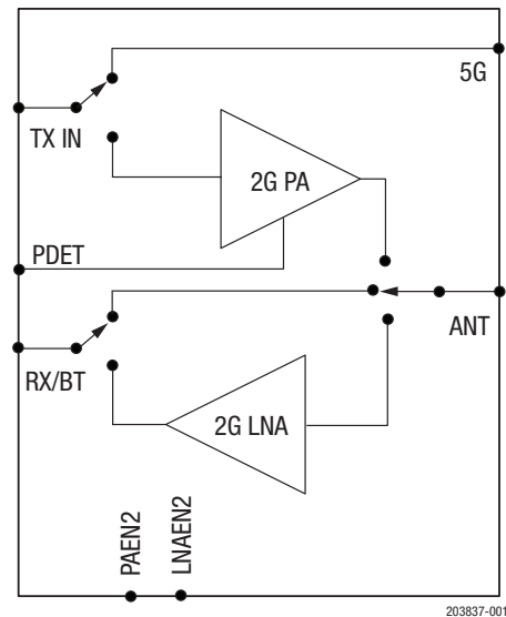
Figure 1. SKY85312-11 Block Diagram
