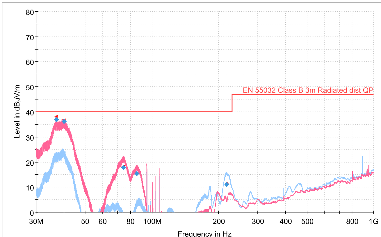
Figure 5.14. Si3404-ISO-FB EVB Radiated Emissions Measurements Results; 50 V Input, 12 V Output, 15 W Input Power
