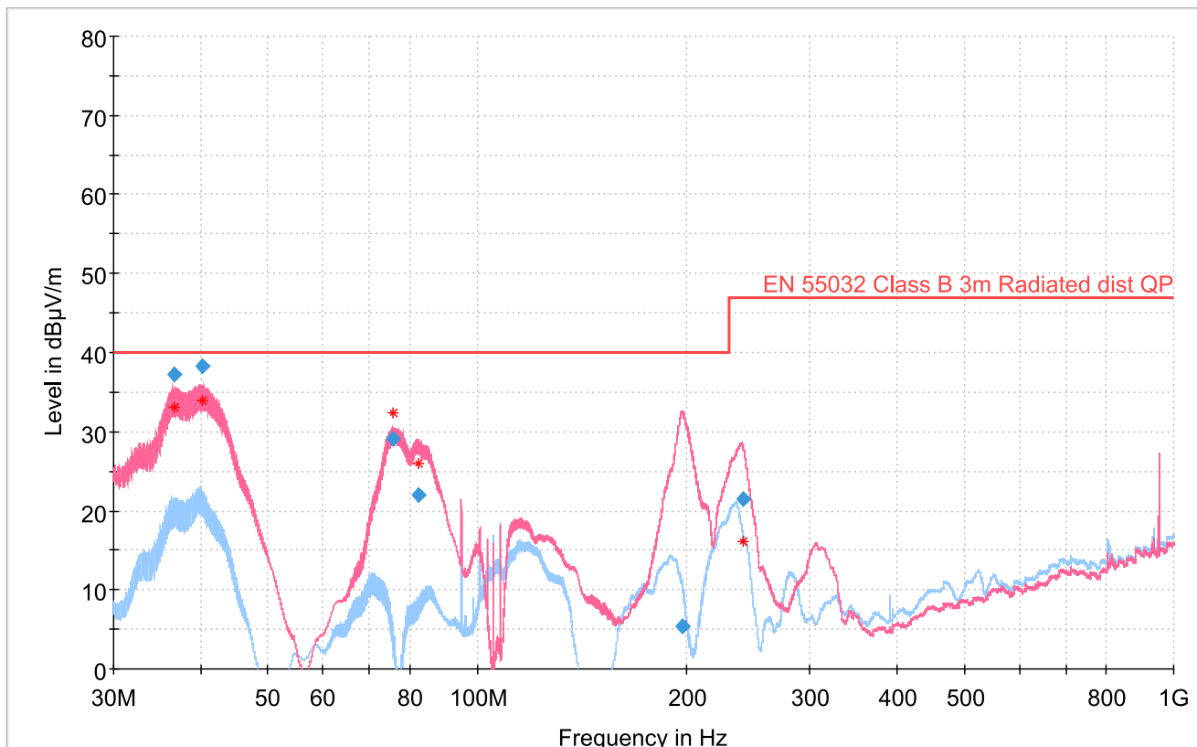
Figure 4.14. Si3404-ISO-FB EVB Radiated Emissions Measurements Results; 50 V Input, 5 V Output, 15 W Input Power
