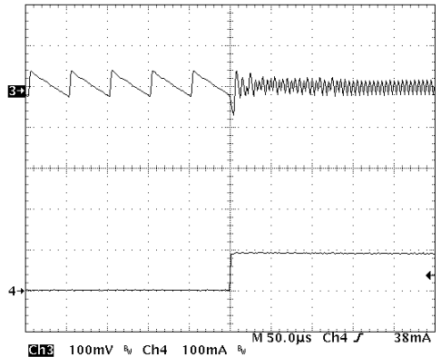
Upper Trace: Output Voltage Ripple, 100 mV/Division Lower Trace: Load Current, I_{LOAD} , 100 mA/Division ( V_{OUT} = 1.8\text{ V} , I_{LOAD} = 10\text{ mA to } 100\text{ mA} ; L = 5.6\text{ }\mu\text{H} , C_{OUT} = 22\text{ }\mu\text{F} )
