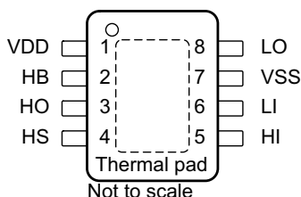
Figure 4-1. DDA Package 8-Pin SO-PowerPAD Top View
