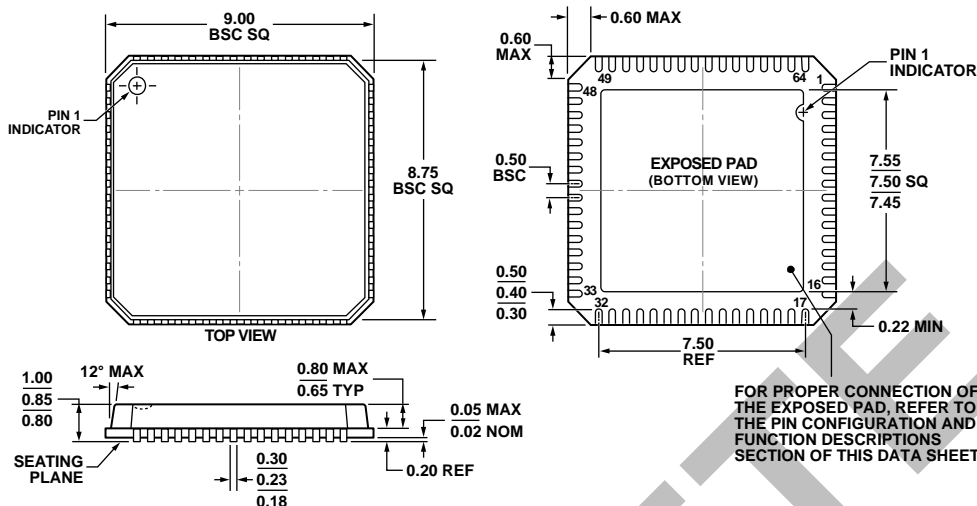
COMPLIANT TO JEDEC STANDARDS MO-220-VMM4 Figure 91. 64-Lead Lead Frame Chip Scale Package [LFCSP_VQ] 9 mm × 9 mm Body, Very Thin Quad (CP-64-6) Dimensions shown in millimeters
