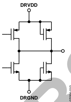
Figure 10. Digital Output
