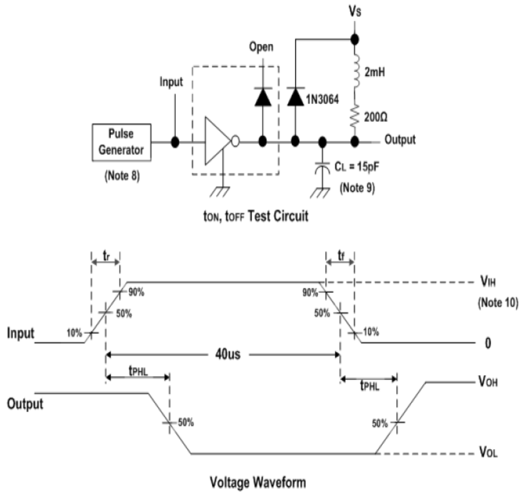
Fig. 9 Latch-Up Test Circuit and Voltage Waveform
