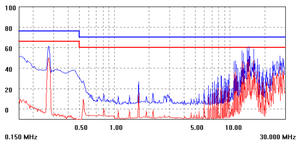
Figure 21. EMC considerations.
