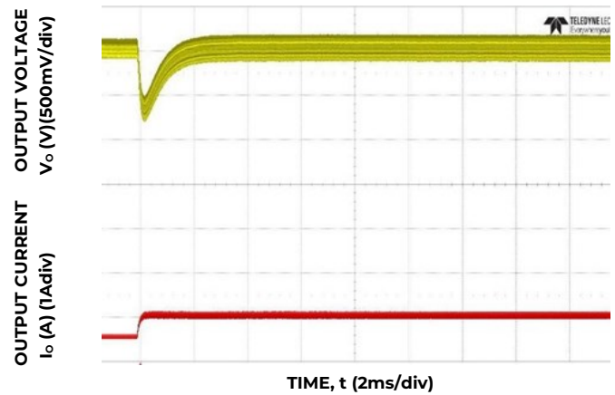
Figure 16. Transient Response to Dynamic Load Change from 0.65A to 1.15A at 12V in , C out =9x4.7µF, C Tune =220pF, R Tune =40.2kΩ
