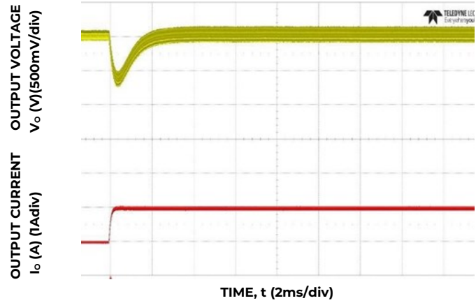
Figure 4. Transient Response to Dynamic Load Change from 50% to 100% at 12V_{in} , C_{out} = 12 \times 4.7\mu\text{F} , C_{Tune} = 820\text{pF} , R_{Tune} = 30.1\Omega
