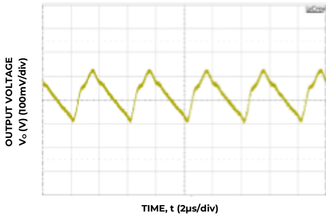
Figure 3. Typical output ripple ( C_o=66\mu\text{F} ceramic, V_{IN} = 12V , I_o = I_{o,max} ).
