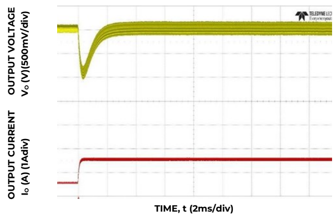
Figure 10. Transient Response to Dynamic Load Change from 0.6 to 1.6A at 12Vin, C out =10x4.7uF, C Tune =560pF, R Tune =40.2k
