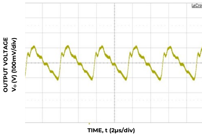
Figure 9. Typical output ripple and noise (C o =66μF ceramic, V IN =12V, I o = I o,max ).
