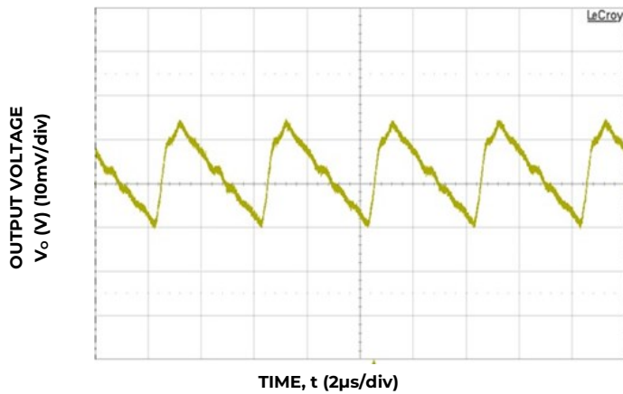
Figure 15. Typical output ripple and noise (C o =66µF ceramic, V IN = 12V, I o = I o,max ).
