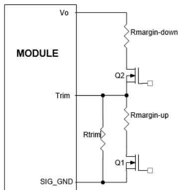
Figure 31. Circuit Configuration for margining Output voltage.
