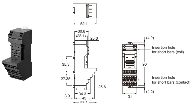
Terminal Arrangement/ Internal Connection Diagram (TOP VIEW)
