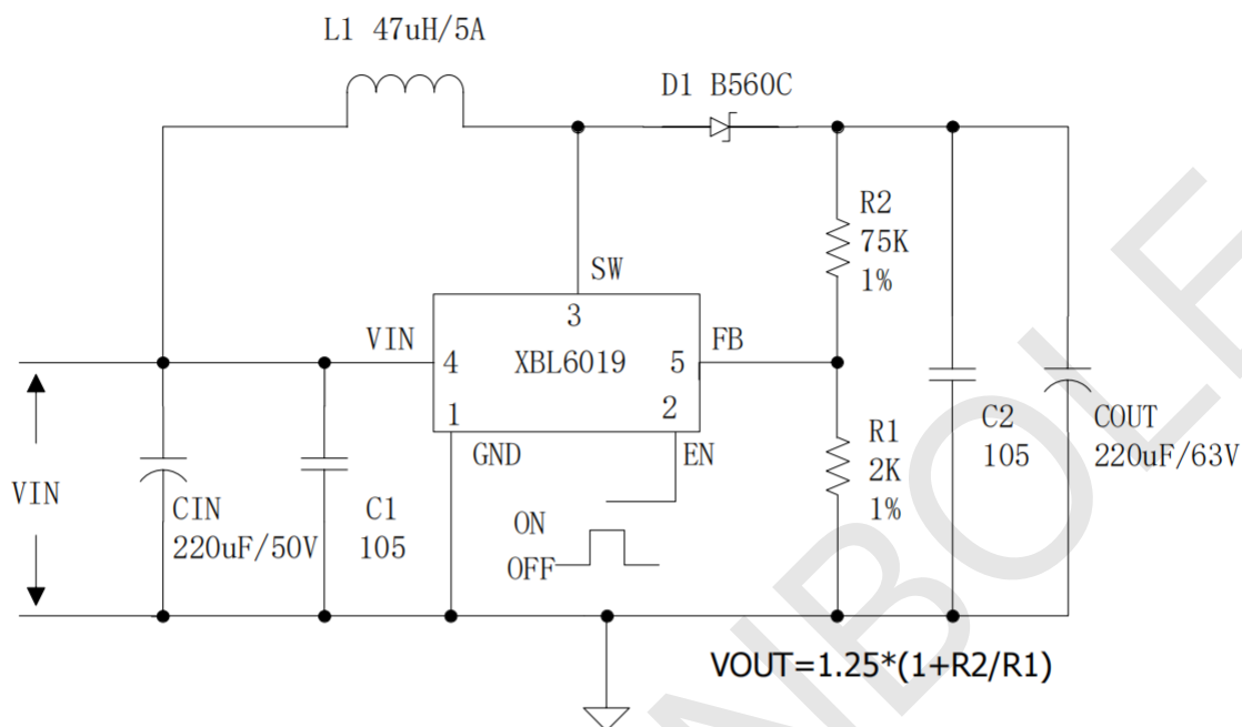
Figure 14. XBL6019 System Parameters Test Circuit (VIN=20~40V,VOUT=48V)
