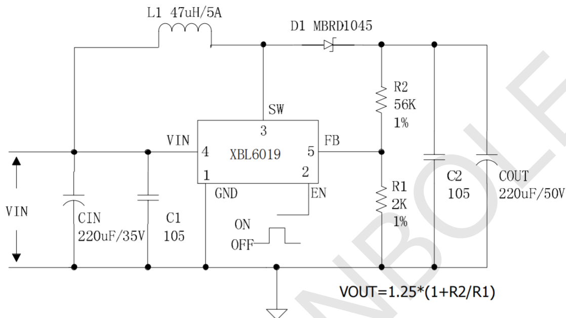
Figure 12. XBL6019 System Parameters Test Circuit (VIN=10~32V,VOUT=36V)
