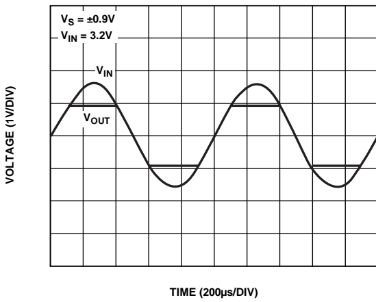
Figure 27. No Phase Reversal
