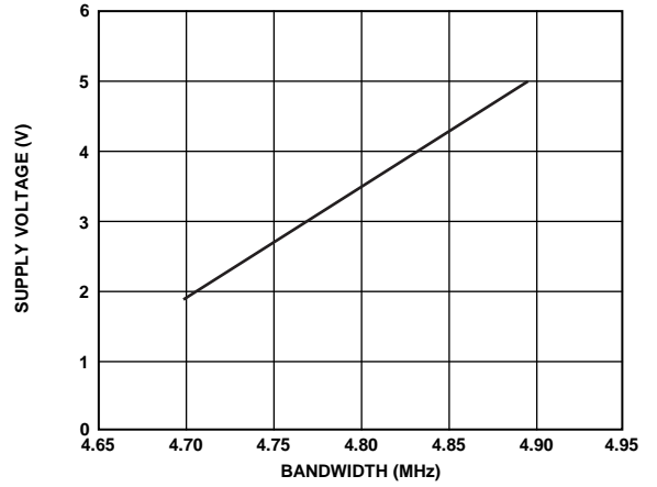
Figure 5. Supply Voltage vs. Bandwidth
