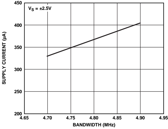
Figure 2. Supply Current vs. Bandwidth
