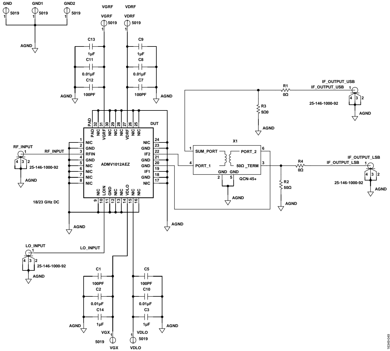
Figure 34. Typical Application Circuit
