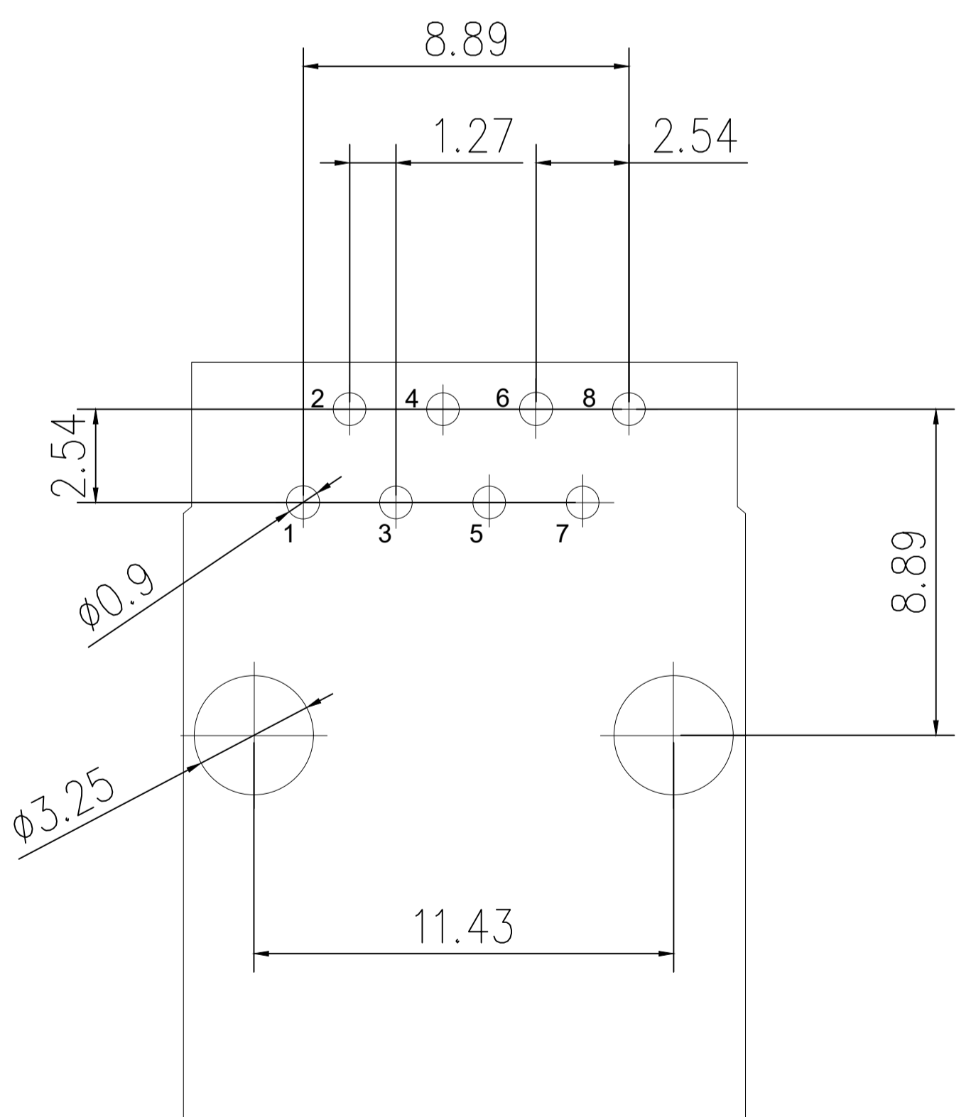
PCB LAYOUT TOP VIEW
