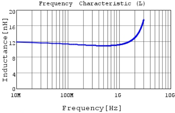
LQP03TN11NH02 L
