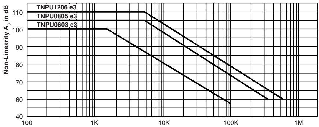
Non-Linearity
