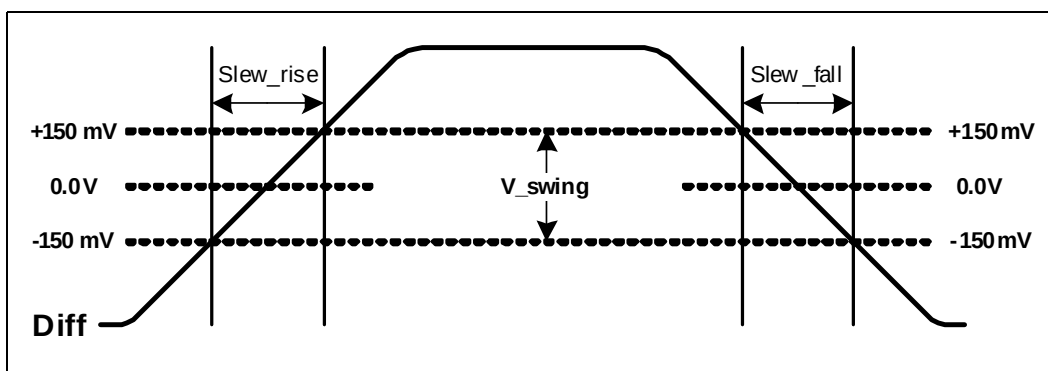
Figure 5. Differential Measurements
