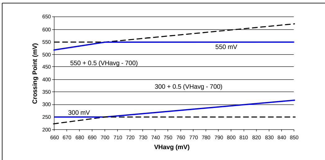
Figure 5. Differential Measurements
