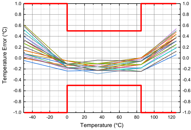
Temperature Error vs. Temperature (3.3V, DFN-2 Package)
