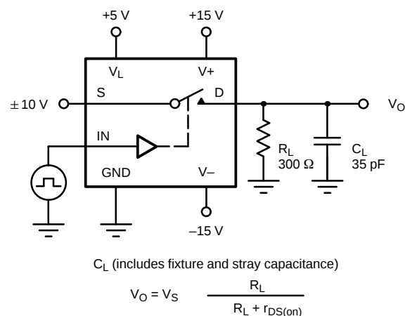
FIGURE 2. Switching Time
