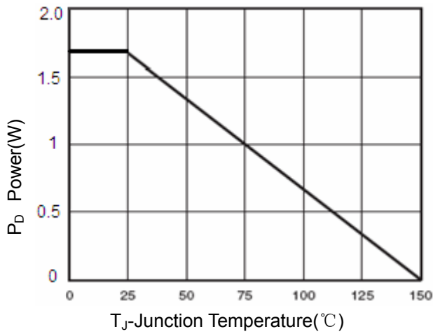
Figure 3 Power Dissipation
