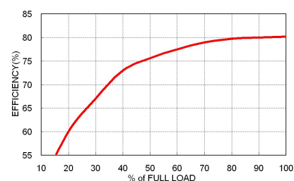
PDL03-48S05 Efficiency vs. Output Load
