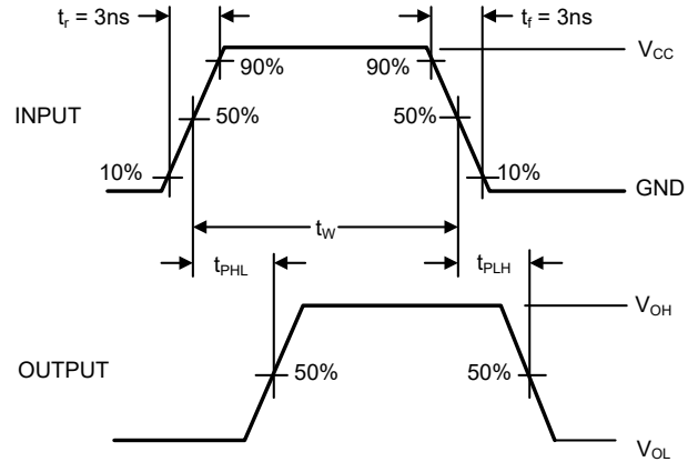
Figure 2. AC Waveforms
