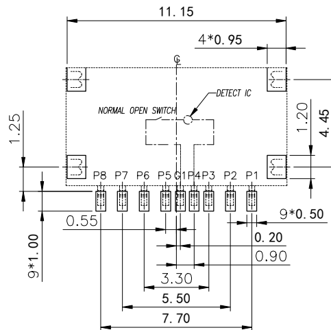
RECOMMEND PCB LAYOUT (TOLERANCE: ±0.05)
