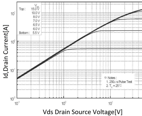
On-Region Characteristics
