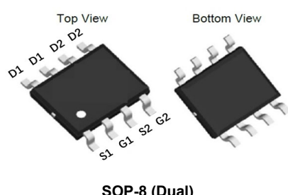
SOP-8 (Dual)
