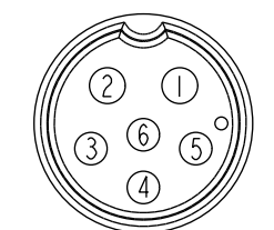
C1 & C2 Pin Assignments Front View
