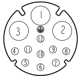
C1 & C2 Pin Assignments Front View
